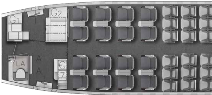
Typical starting configuration with G7 Galley
