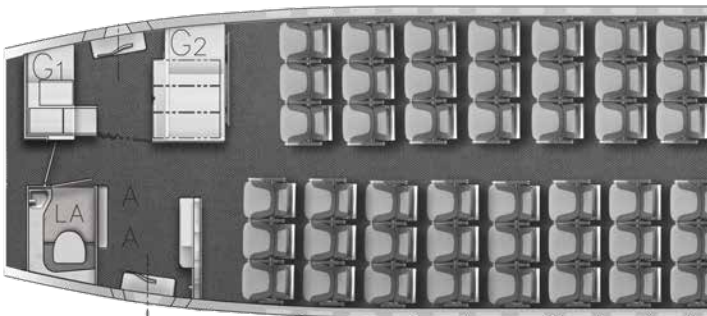
Replace G7 Galley with 737 Door One Windscreen. Note that seat reconfiguration is a separate modification.
